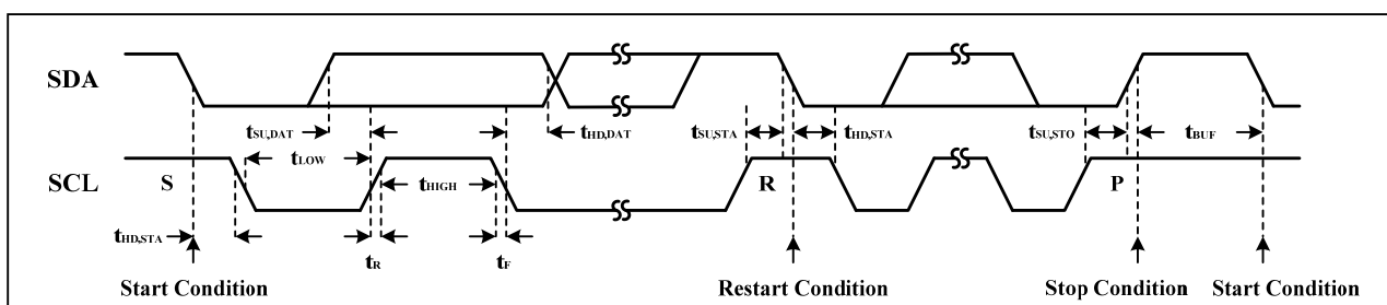
Figure 2 Interface timing
