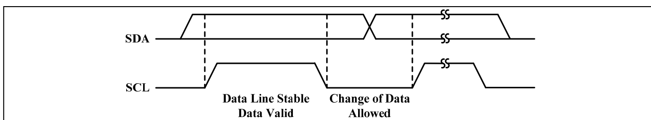
Figure 3 Bit transfer
