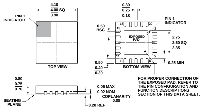
Figure 29. 20-Lead Lead Frame Chip Scale Package [LFCSP_WQ] 4 mm × 4 mm Body, Very, Very Thin Quad (CP-20-8) Dimensions shown in millimeters
