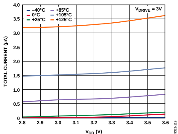
Figure 18. Full Shutdown Current vs. Supply Voltage for Various Temperatures
