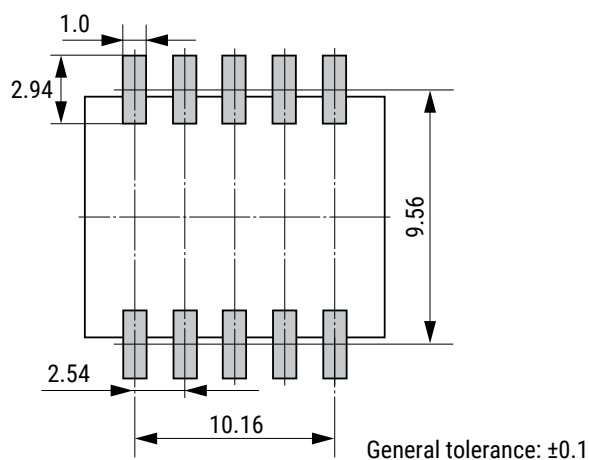
EB2 (bottom view)
