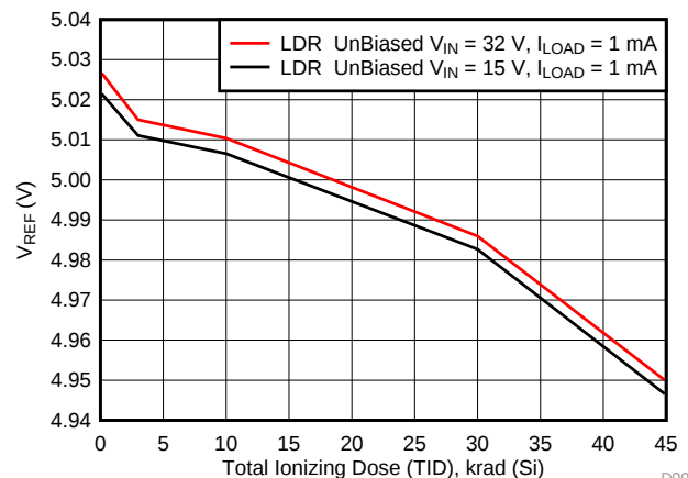
V_{REF} Radiation Drift Curve
