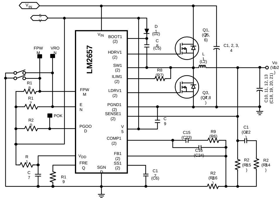
Figure 20. High Current Application Circuit
