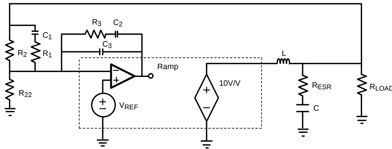
Figure 16. LM2657 Closed Loop Model with Type 3 Compensation
