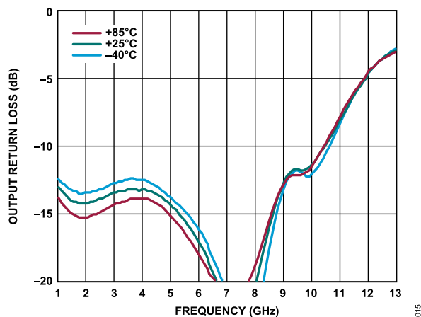
Figure 15. Output Return Loss vs. Frequency for Various Temperatures, 1 GHz to 13 GHz, V_{DD} = 5 V, I_{DQ} = 60 mA, R_{BIAS} = 1.47 k \Omega
