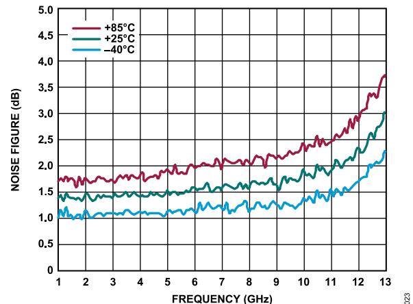
Figure 23. Noise Figure vs. Frequency for Various Temperatures, 1 GHz to 13 GHz, V_{DD} = 5 V, I_{DQ} = 60 mA, R_{BIAS} = 1.47 kΩ
