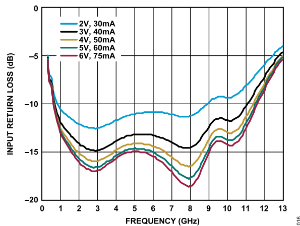
Figure 16. Input Return Loss vs. Frequency for Various V_{DD} and I_{DQ} Values, 300 MHz to 13 GHz, R_{BIAS} = 1.47 k \Omega
