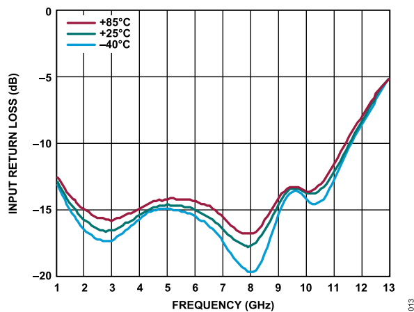
Figure 13. Input Return Loss vs. Frequency for Various Temperatures, 1 GHz to 13 GHz, V_{DD} = 5 V, I_{DQ} = 60 mA, R_{BIAS} = 1.47 k \Omega
