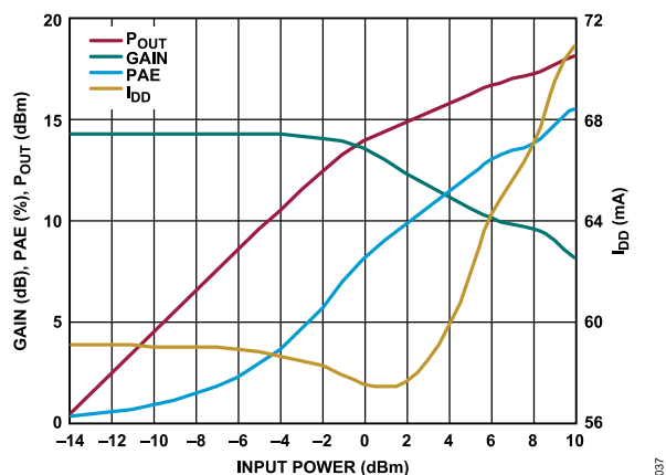
Figure 37. Gain, PAE, P_{OUT} , and I_{DD} vs. Input Power, Power Compression at 10 GHz, V_{DD} = 5 V, I_{DQ} = 60 mA, R_{BIAS} = 1.47 k \Omega
