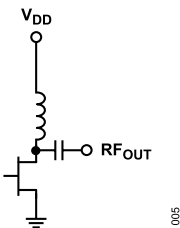
Figure 5. VDD and RFOUT Interface Schematic
