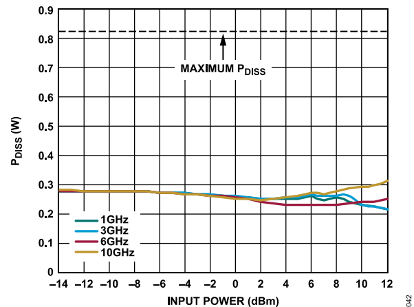
Figure 42. P_{DISS} vs. Input Power at T_A = 85^\circ\text{C} , V_{DD} = 5 V, I_{DQ} = 60 mA, R_{BIAS} = 1.47 k \Omega
