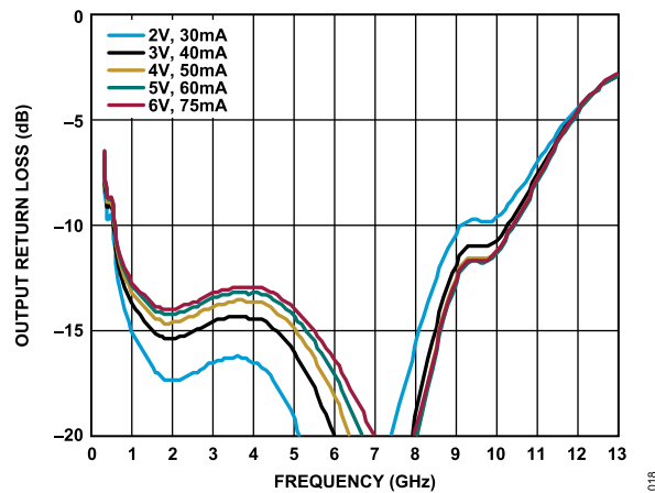
Figure 18. Output Return Loss vs. Frequency for Various V_{DD} and I_{DQ} Values, 300 MHz to 13 GHz, R_{BIAS} = 1.47 k \Omega
