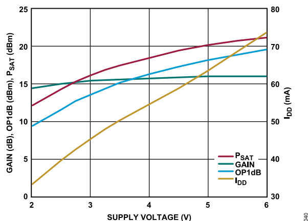
Figure 40. Gain, OP1dB, P_{SAT} , and I_{DD} vs. Supply Voltage, Power Compression at 1 GHz, R_{BIAS} = 1.47 k \Omega
