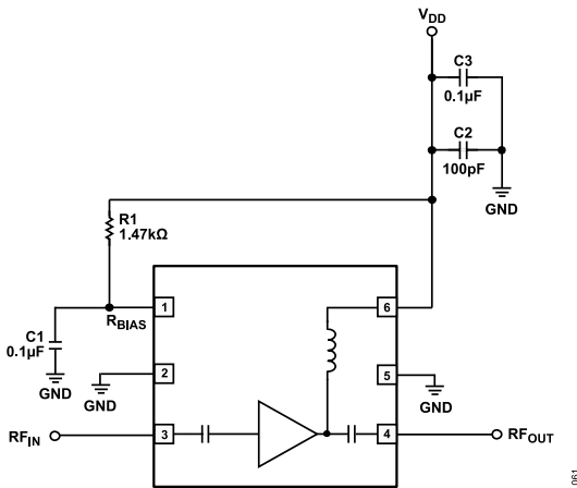
Figure 60. Typical Application Circuit
