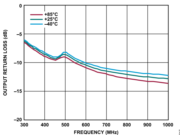
Figure 17. Output Return Loss vs. Frequency for Various Temperatures, 300 MHz to 1 GHz, R_{BIAS} = 1.47 k \Omega
