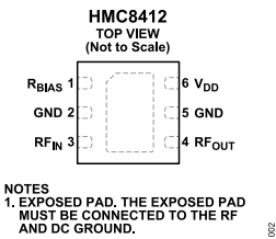
Figure 2. Pin Configuration
