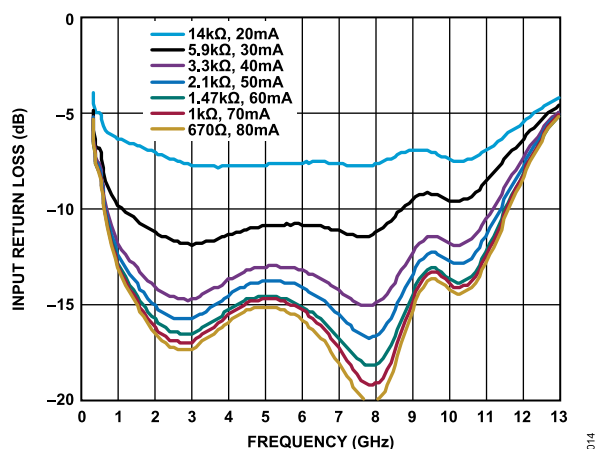
Figure 14. Input Return Loss vs. Frequency for Various R_{BIAS} Values and I_{DQ} , 300 MHz to 13 GHz, V_{DD} = 5 V
