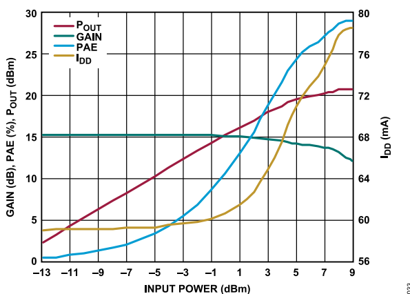
Figure 33. Gain, PAE, P_{OUT} , and Drain Current ( I_{DQ} ) vs. Input Power, Power Compression at 3 GHz, V_{DD} = 5\text{ V} , I_{DQ} = 60\text{ mA} , R_{BIAS} = 1.47\text{ k}\Omega
