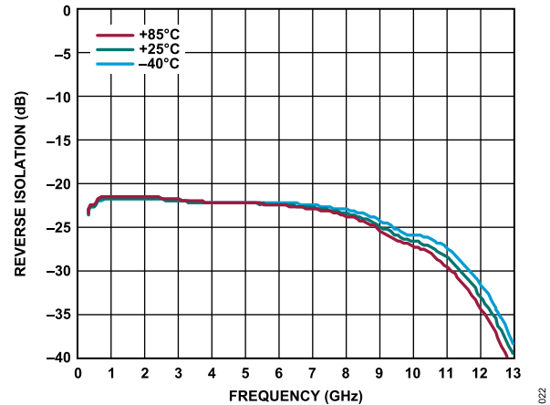
Figure 22. Reverse Isolation vs. Frequency for Various Temperatures, 300 MHz to 13 GHz, V_{DD} = 5 V, I_{DQ} = 60 mA, R_{BIAS} = 1.47 kΩ
