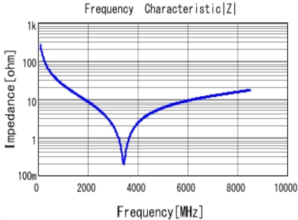
■ GCQ1555C1H6R2WB01 |Z| DC0V, 25degC
