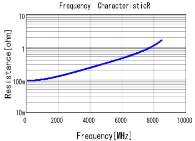
■ GCQ1555C1H6R2WB01 R DC0V, 25degC
