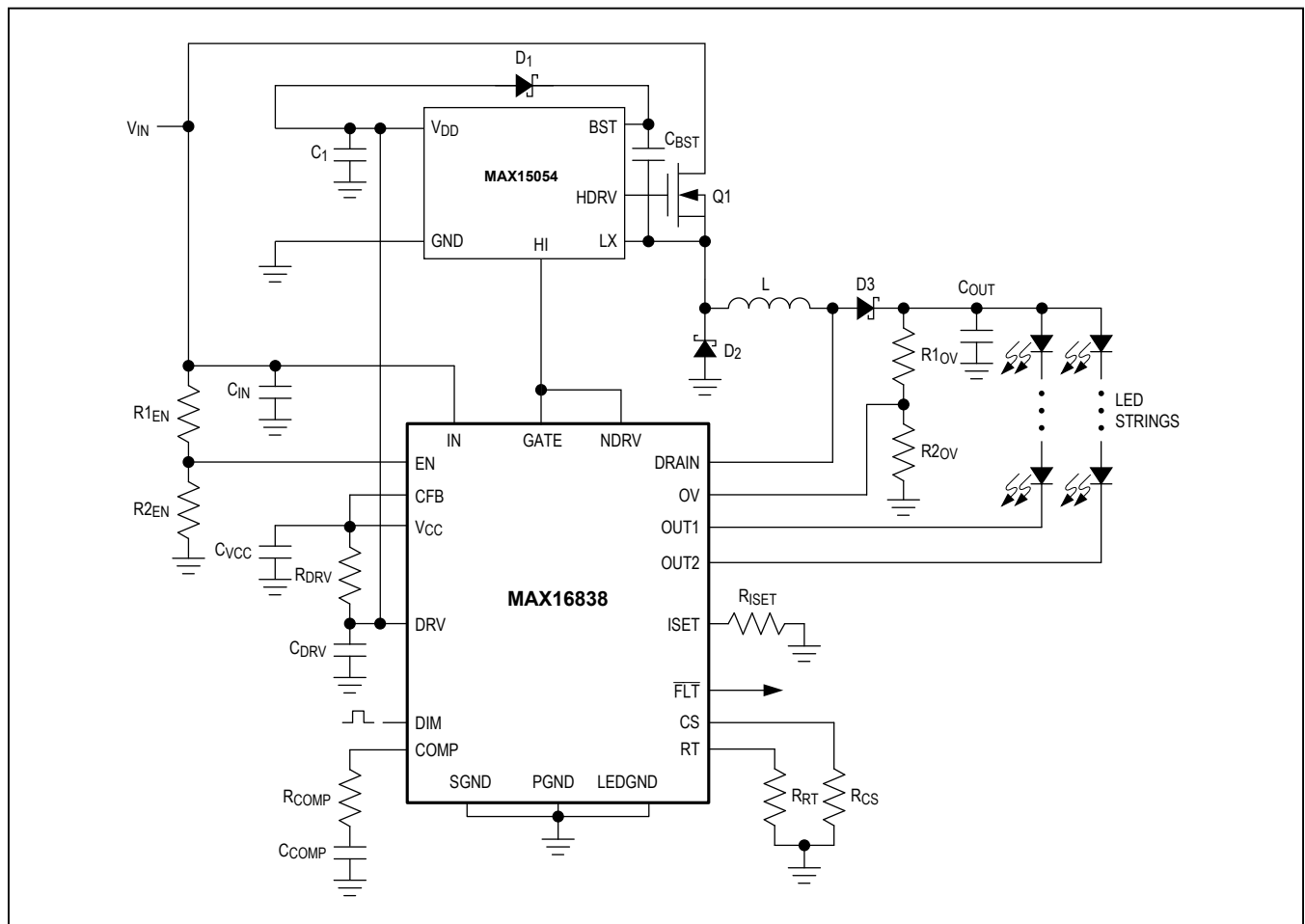
Figure 5. Boost-Buck Configuration
