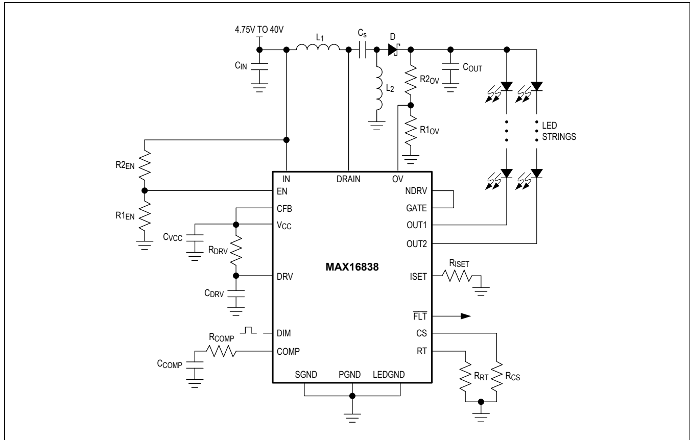
Figure 4. SEPIC Configuration
