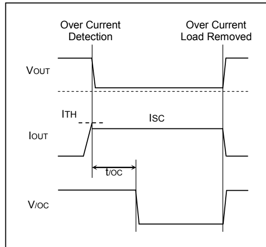
Figure 41. Over-Current Detection
