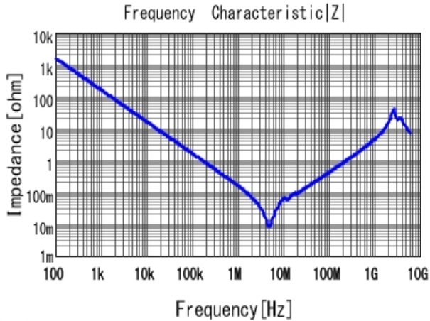
■ GRM55RR71H105KA01 |Z| DC0V, 25degC
