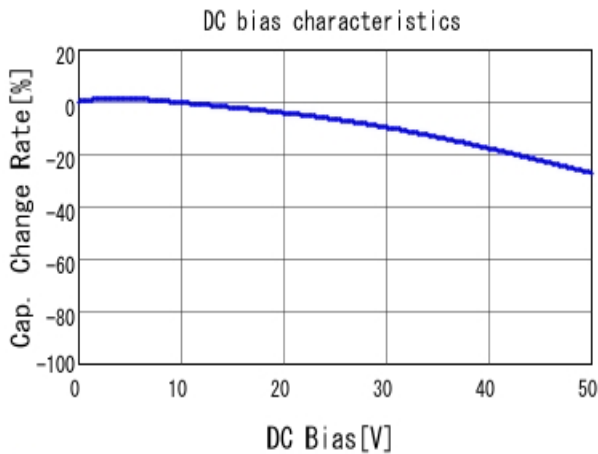
■ GRM55RR71H105KA01 C-DC bias capchange, 25.0degC, AC1.
