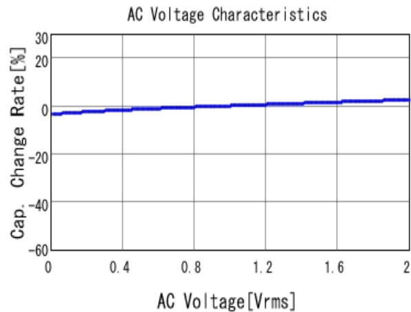
■ GRM55RR71H105KA01 C-AC Voltage capchange, DC0V, 25.0d
