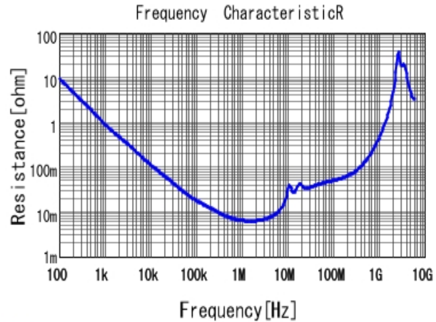
■ GRM55RR71H105KA01 R DC0V, 25degC
