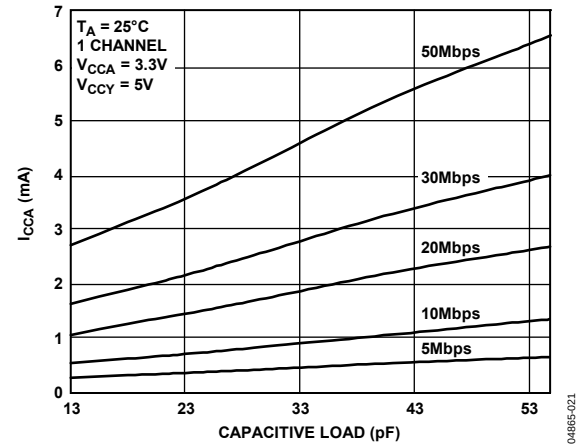
Figure 14. I_{CCA} vs. Capacitive Load at Pin A for Y→A (5 V→3.3 V) Level Translation
