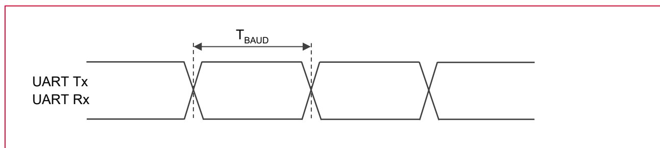
Figure 15: High Speed UART Timing Diagram
