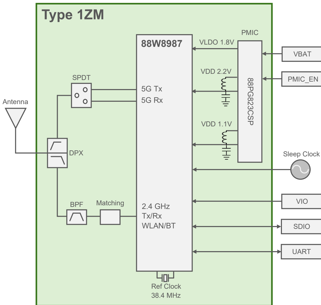
Figure 1: Block Diagram
