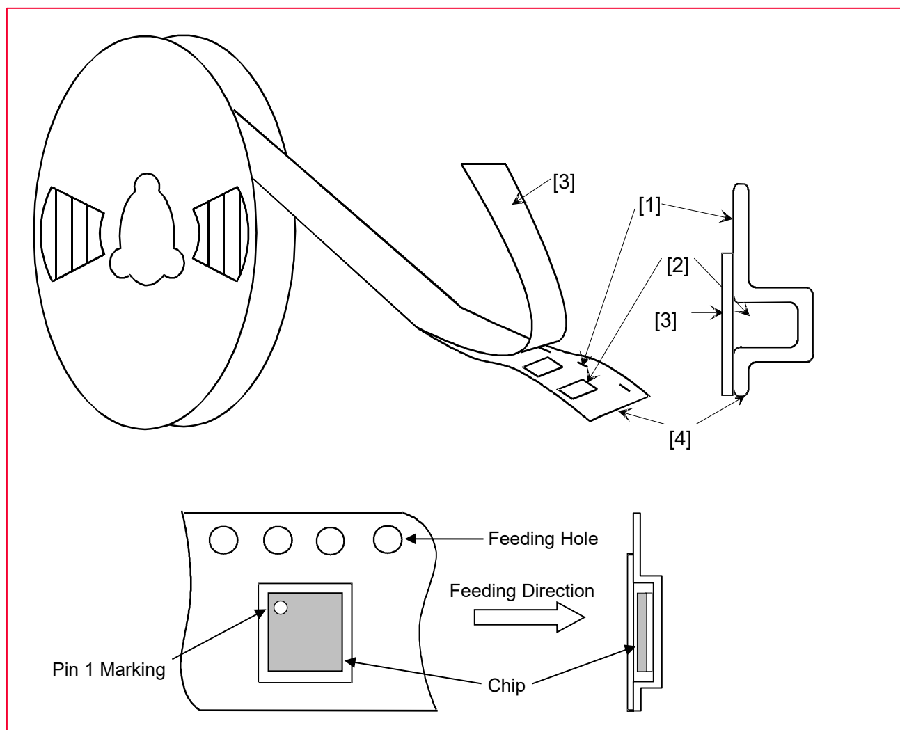
Figure 27: Taping Diagrams
