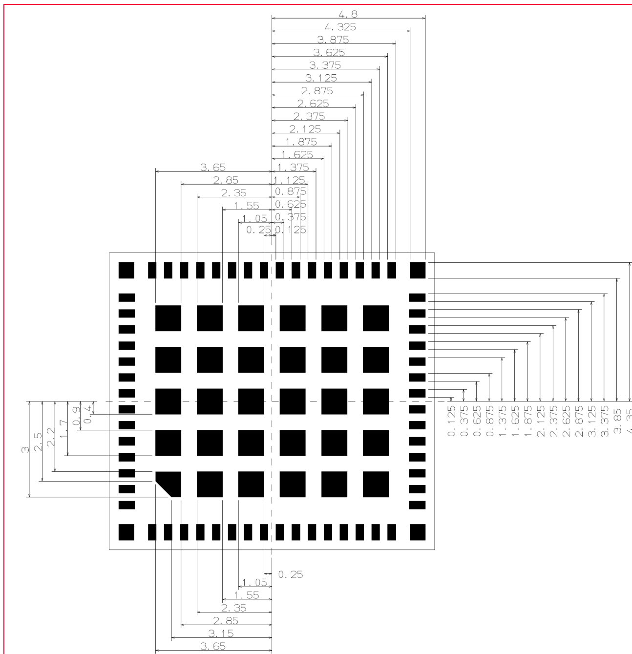
Figure 21: Land Patterns
