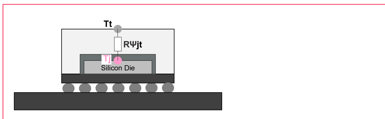
Figure 6: Package Thermal Conditions
