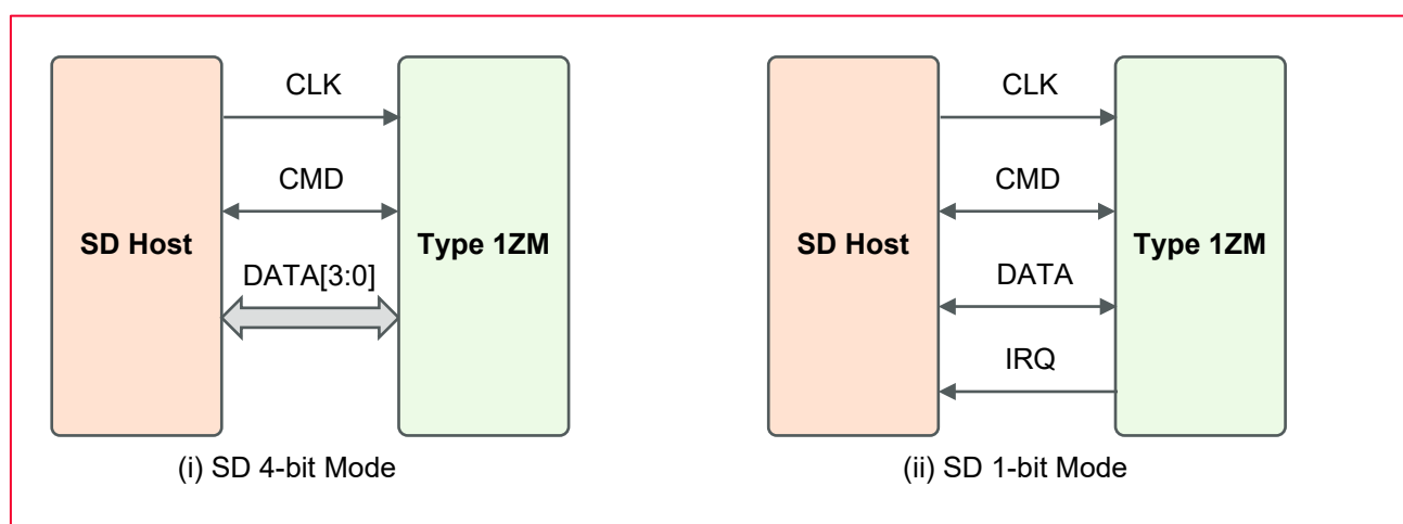
Figure 5: SDIO Pins
