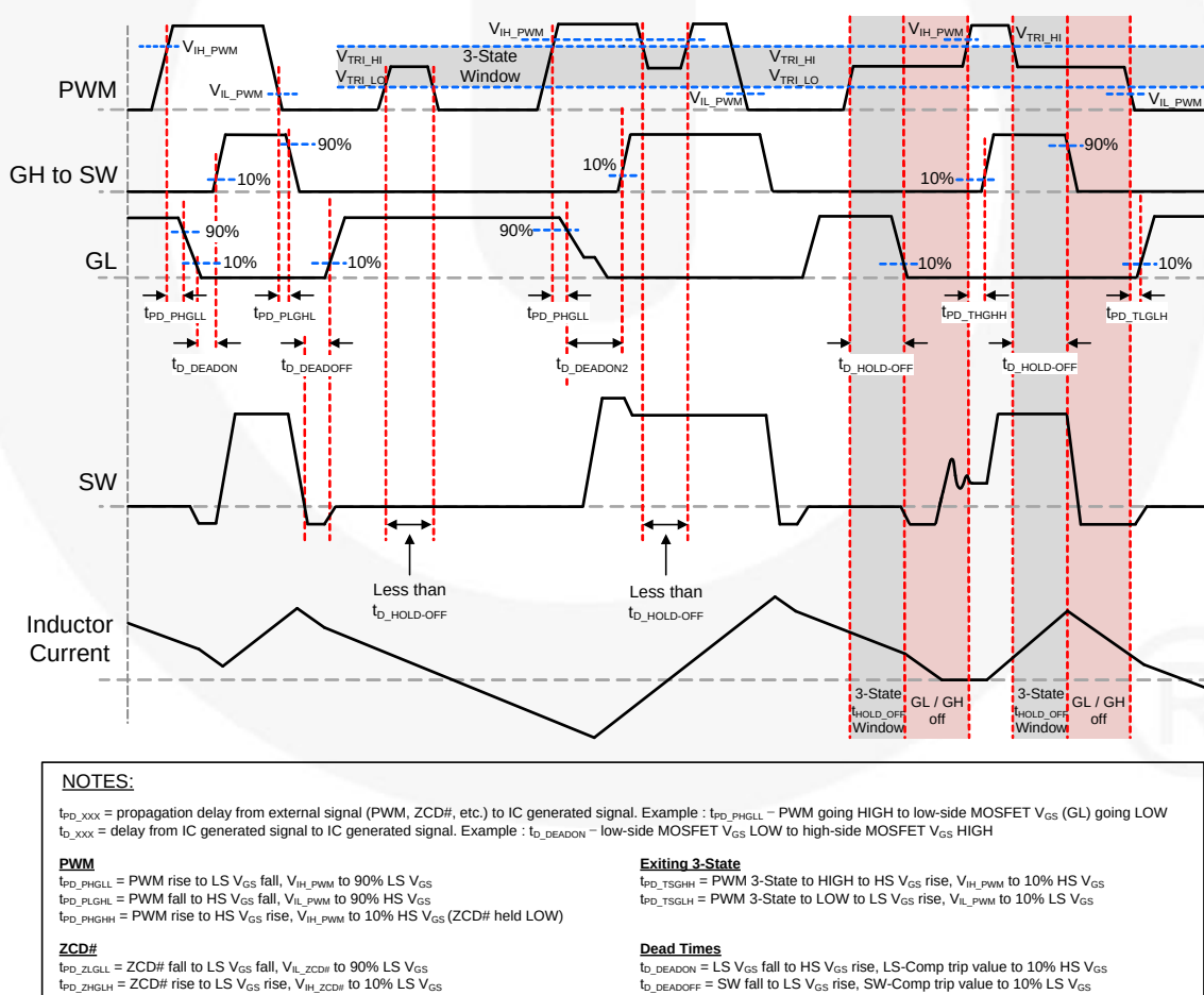
Figure 29. PWM HIGH / LOW / 3-State Timing Diagram
