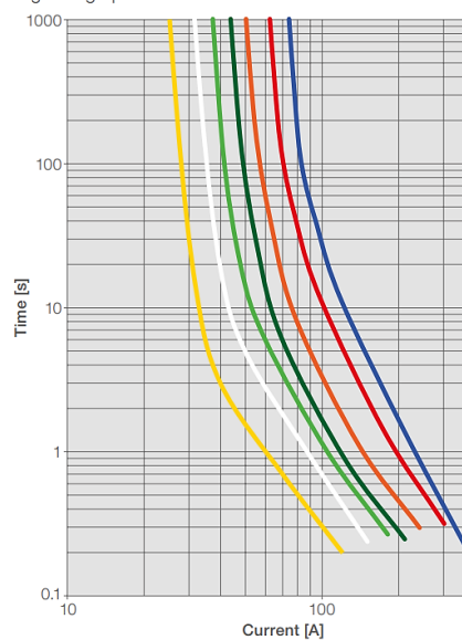
Melting time graph at 23°C on test module ISO.
