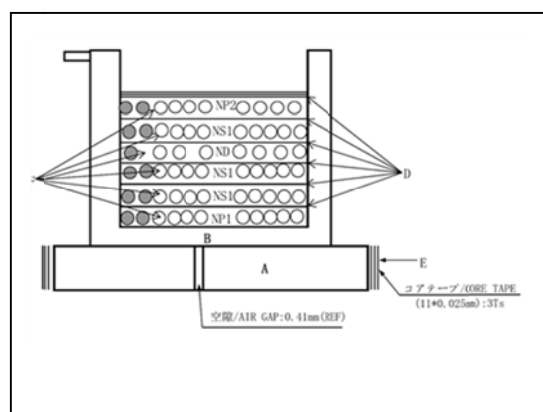
Figure 29. Structure Diagram
