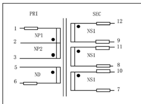
Figure 28. Circuit Diagram
