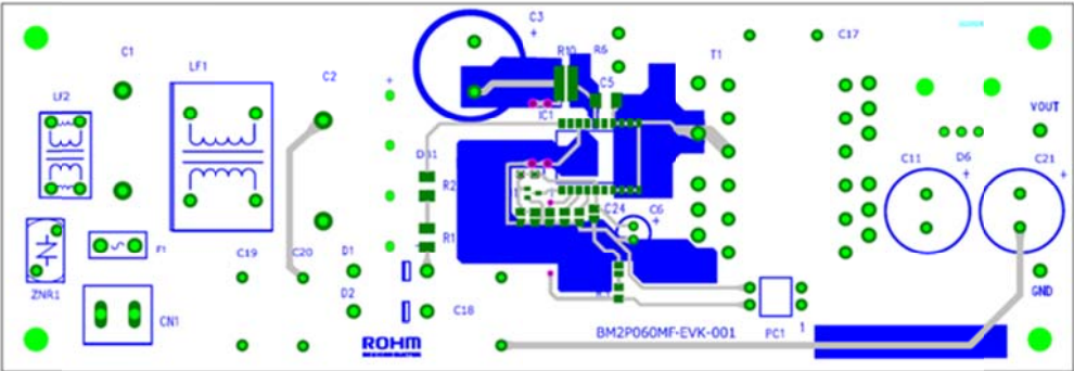
Figure 26. TOP Layout (Top view)
