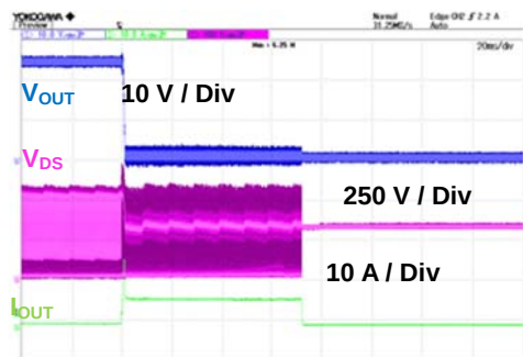
Figure 15. VIN = 90 Vac, VOUT Shorted
