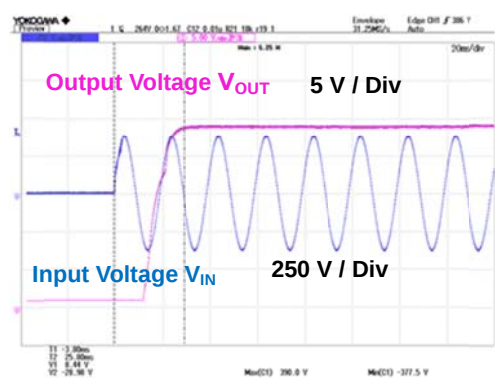
Figure 18. VIN = 264 Vac, IOUT = 1.67 A
