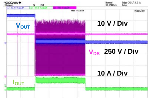
Figure 16. VIN = 264 Vac, VOUT Shorted
