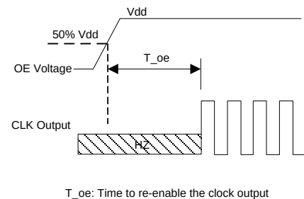
Figure 5. OE Enable Timing (OE Mode Only)
