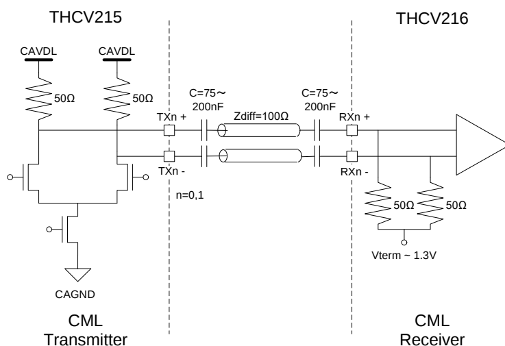
Figure 5. CML buffer scheme
