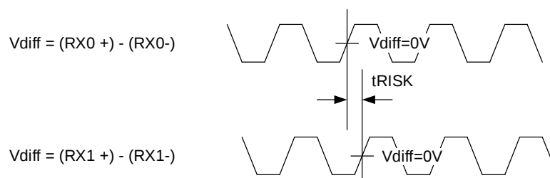
Figure 16. THCV216 CML Input Timing Diagrams
