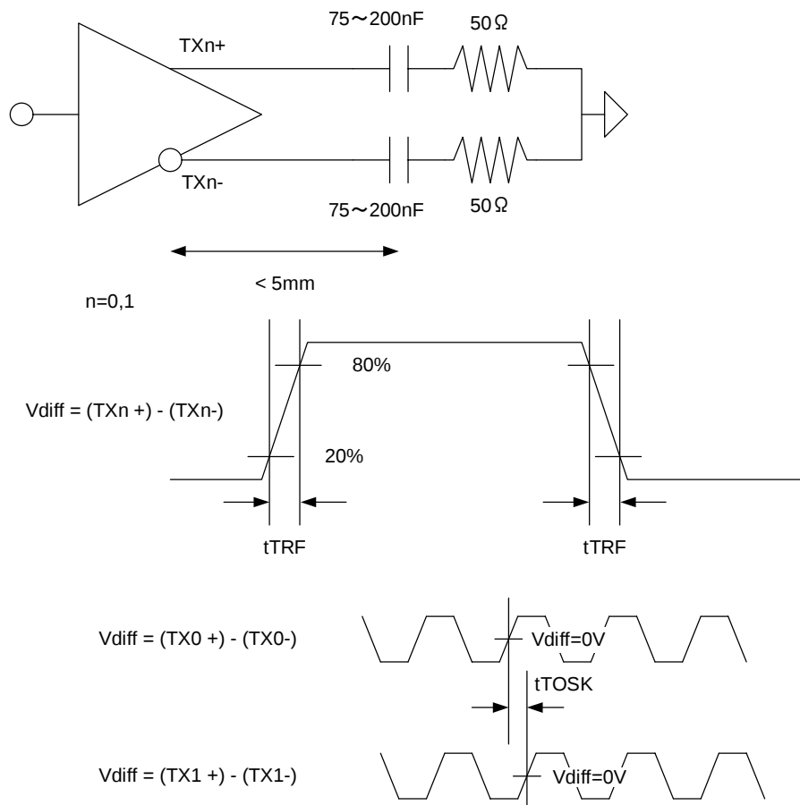
Figure 15. THCV215 CML Output Switching Timing Diagrams and Test Circuit
