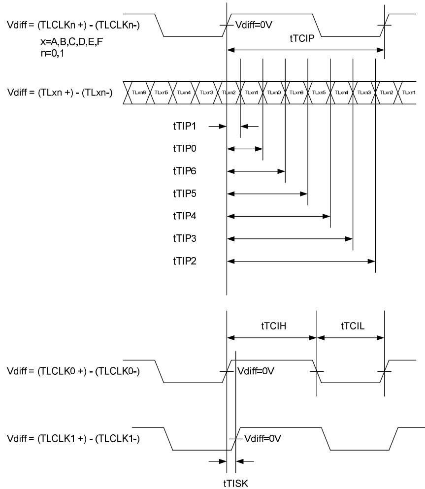
Figure 12. THCV215 LVDS Input Switching Timing Diagrams
