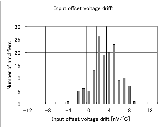
□ Input offset voltage drift(VDD=5V, Ta=25°C, Ta=-40 to 85°C)
