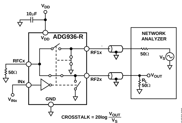
Figure 23. Crosstalk
