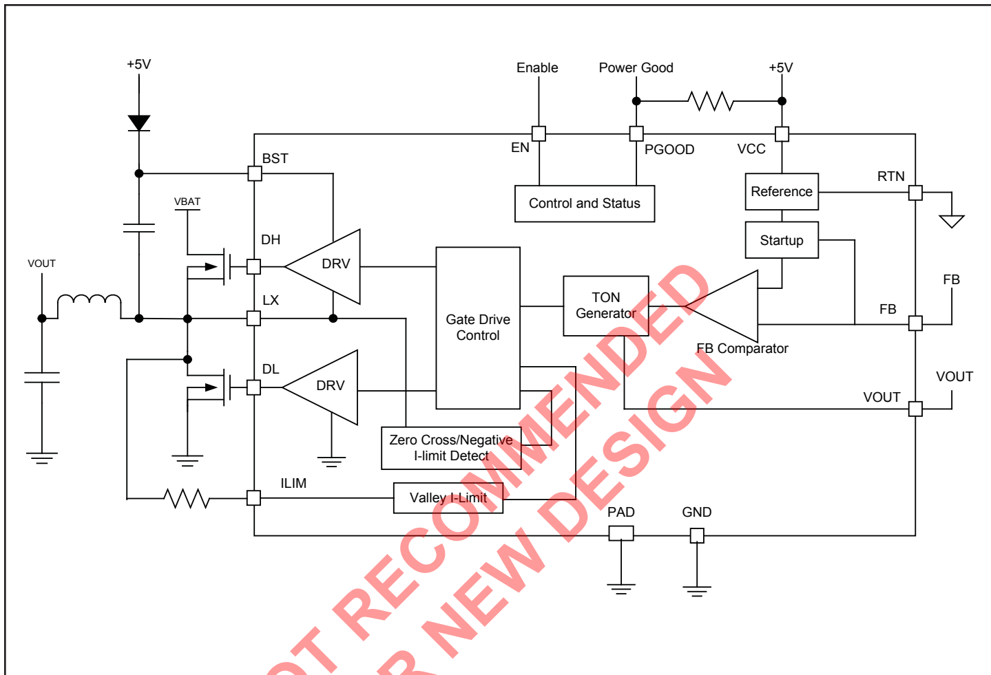
Block Diagram
