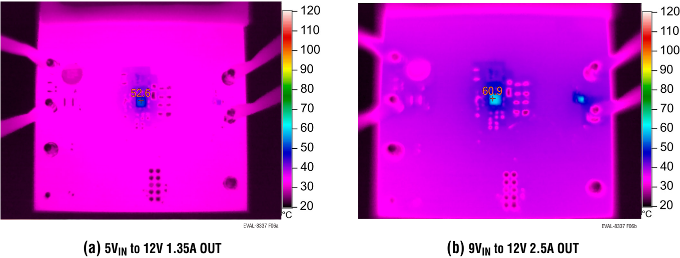
Figure 6. EVAL-LT8337-1-AZ Thermals
