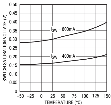
SW Saturation Voltage vs Temperature
