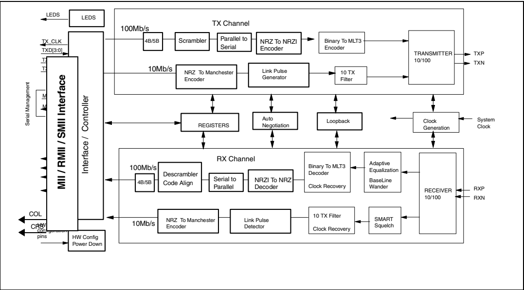
Figure 2. Block diagram
