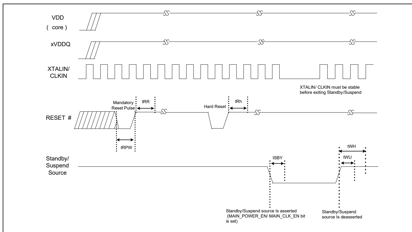
Figure 6 Reset sequence
