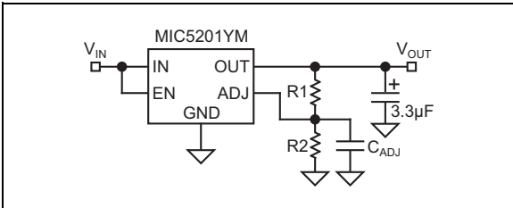
FIGURE 4-3: Decreasing Output Noise.
