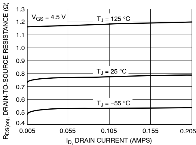
Figure 3. On-Resistance vs. Drain Current and Temperature
