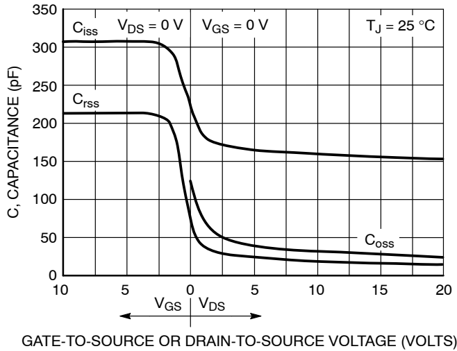
Figure 11. Capacitance Variation
