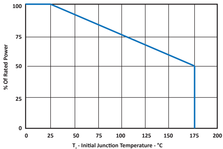
FIGURE 3 POWER DERATING CURVE
