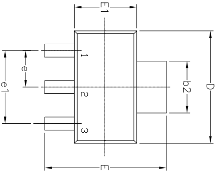
GAUGE PLANE
