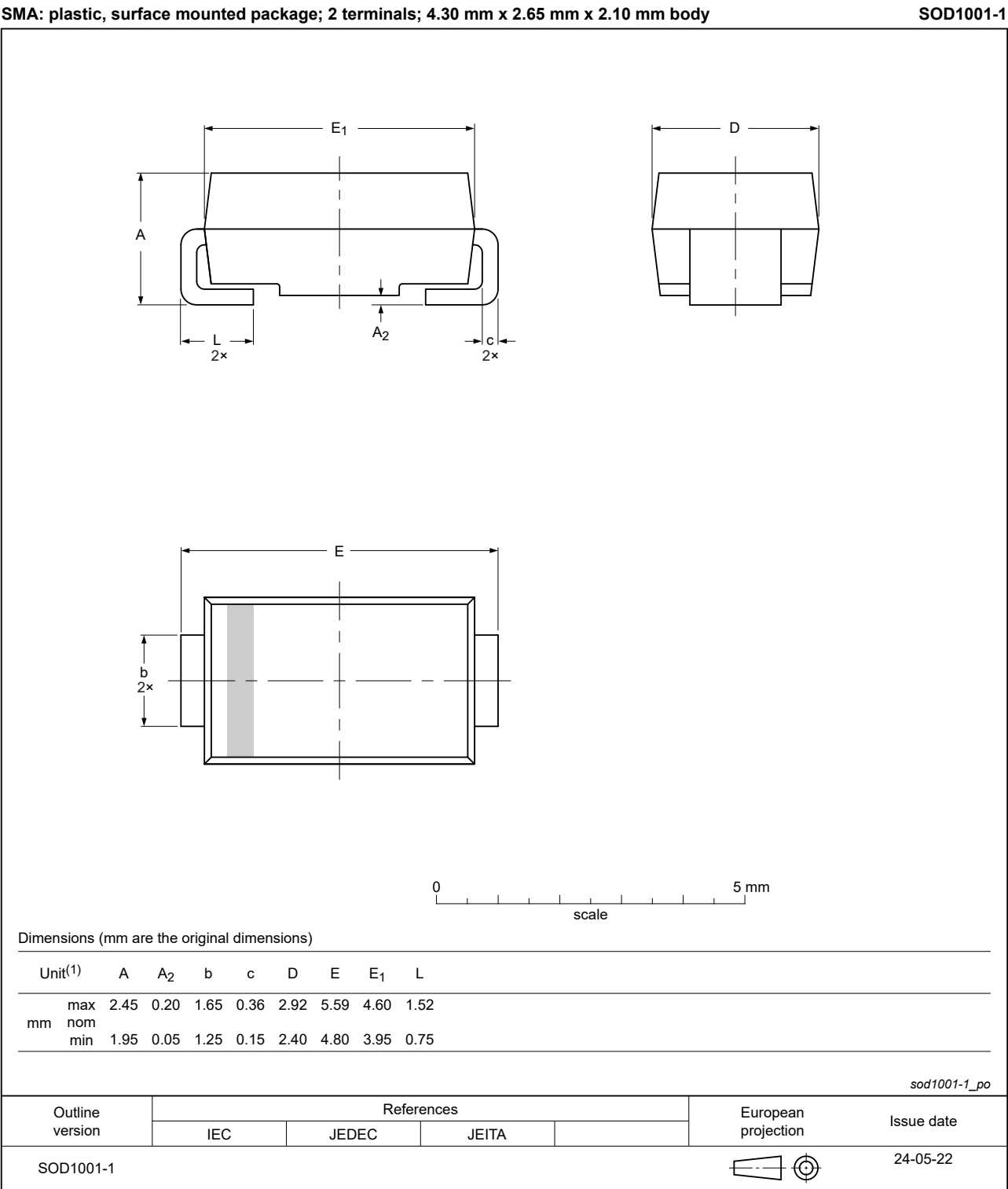
Fig. 8. Package outline SMA (SOD1001-1)
