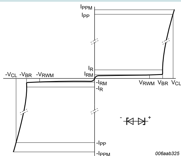
Fig. 6. V-I characteristics for a bidirectional TVS diode
