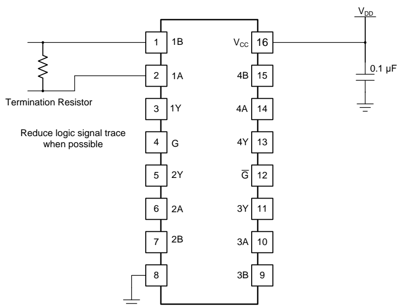
Figure 19. Layout with PCB Recommendations
