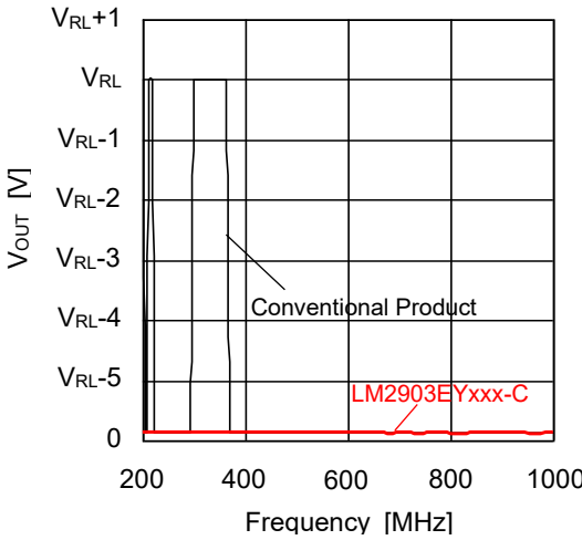
Figure 21. EMI Characteristics (L Level Output)
