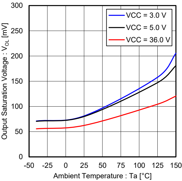
Figure 4. Output Saturation Voltage vs Ambient Temperature (I OL = 4 mA)
