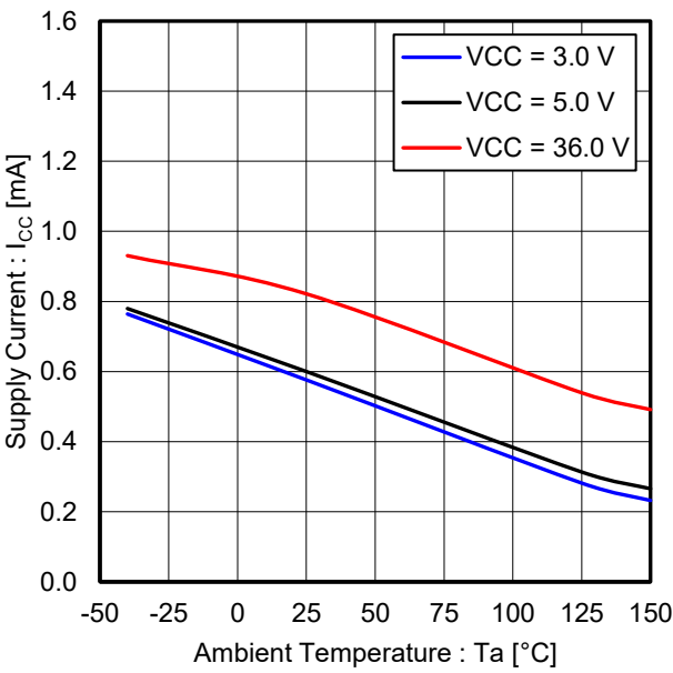
Figure 2. Supply Current vs Ambient Temperature
