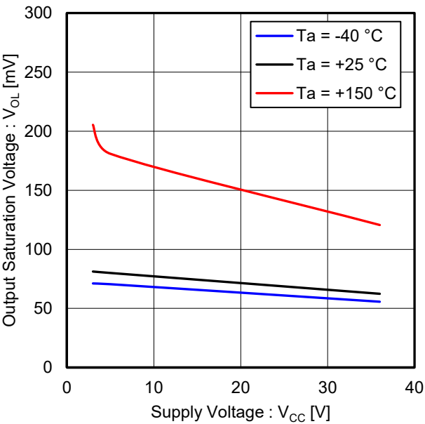
Figure 3. Output Saturation Voltage vs Supply Voltage (I OL = 4 mA)
