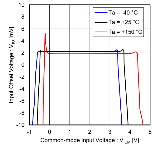
Figure 15. Input Offset Voltage vs Common-mode Input Voltage ( V_{CC} = 5\text{ V} )
