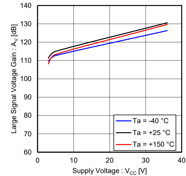
Figure 13. Large Signal Voltage Gain vs Supply Voltage
