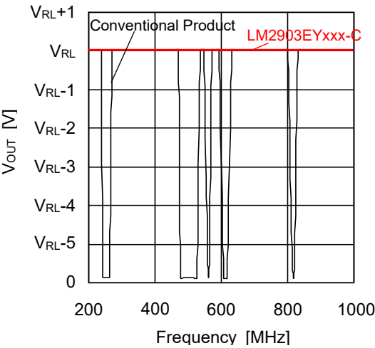
Figure 20. EMI Characteristics (H Level Output)
