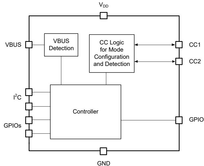
Figure 2. Simplified Schematic
