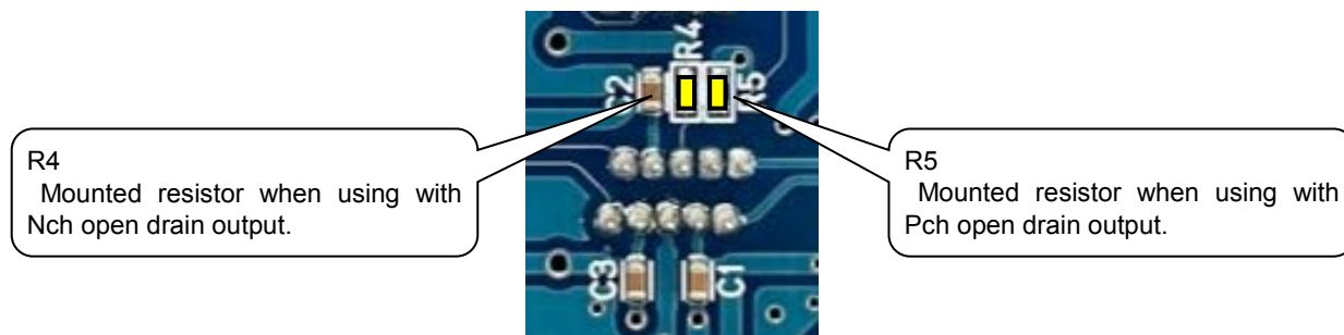
Figure 3 R4,R5 land
