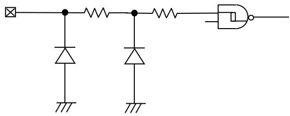
Figure 57. Input pin circuit diagram
