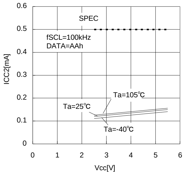
Figure 12. Current consumption at READ operation ICC2 ( f_{SCL}=100\text{kHz} )
