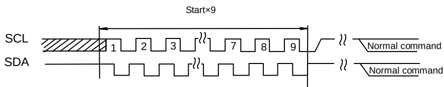
Figure 46-(c) START×9+ command input
