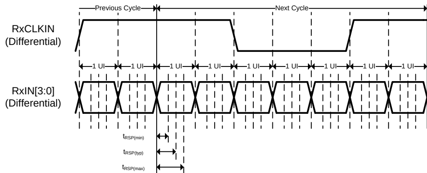
Figure 4. FPD-Link Input Strobe Position
