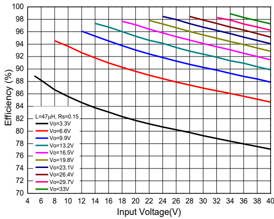
Efficiency vs. Input Voltage (TSOT25, R s =0.15Ω, L=47μH)
