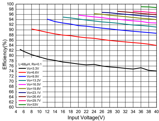
Efficiency vs. Input Voltage (MSOP-8EP, R s =0.1Ω, L=68μH)
