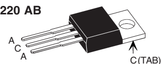
TO-220 AB
