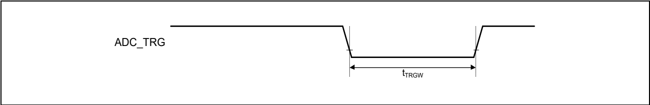
Figure 3.50 ADC Trigger Input Timing
