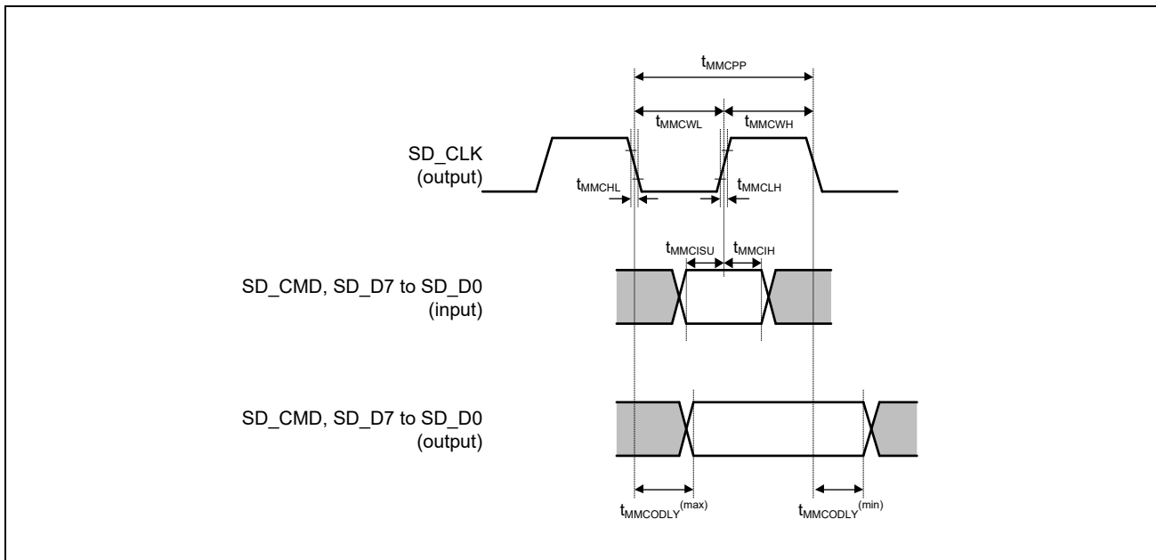
Figure 3.9 eMMC Host Interface Timing (MMC Default/HS-SDR 1.8-V/3.3-V Power Supply)
