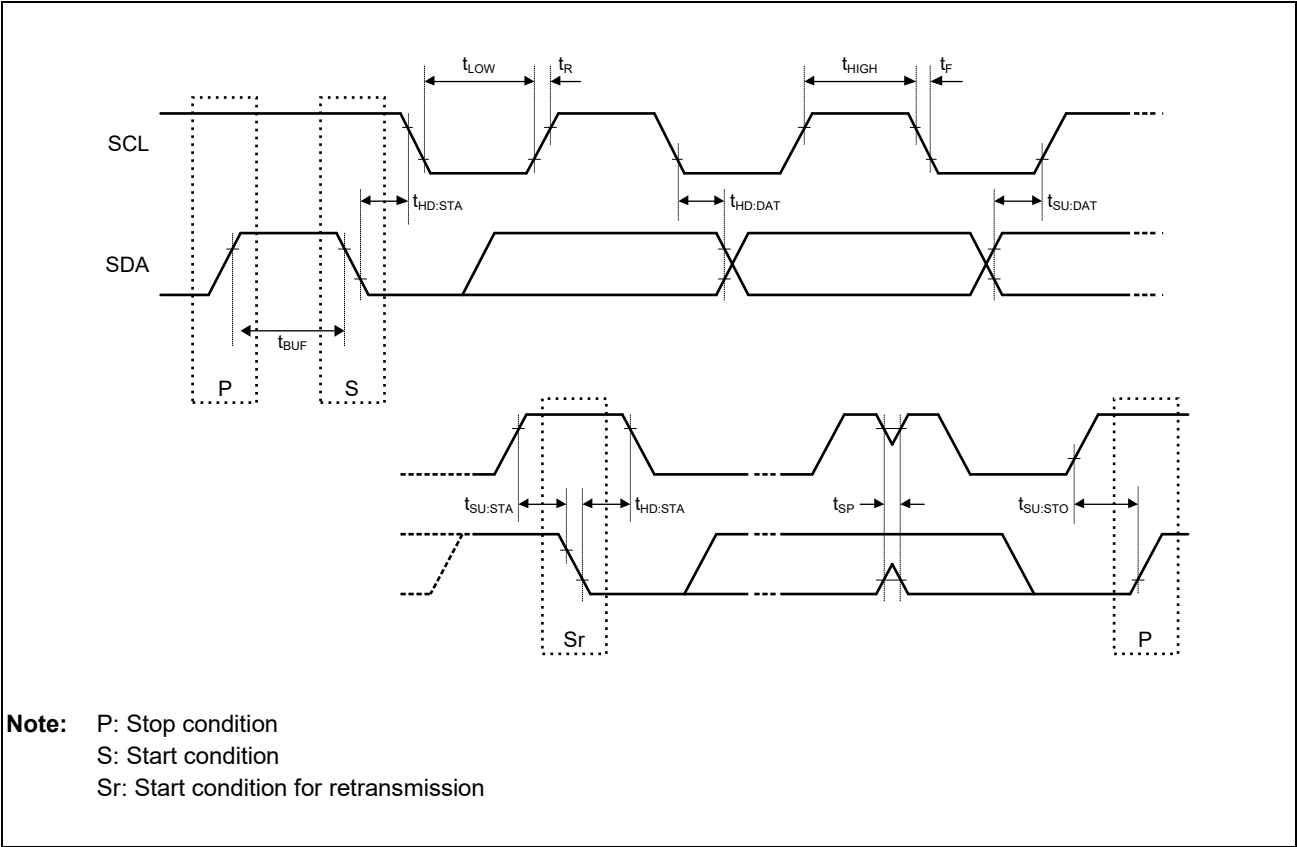
Figure 3.40 Input/Output Timing
