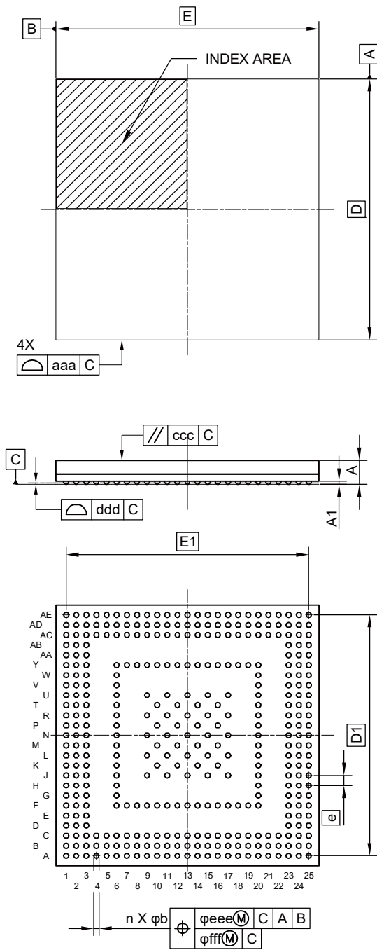
Figure 4.1 Package Dimensions for LFBGA 13 mm□/0.5 mm pitch/361 pin
