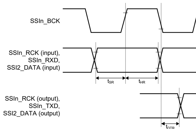
Figure 3.33 Transmission and Reception Timing (SSIBCK Falling Output)
