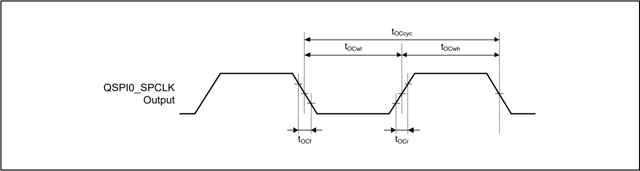
Figure 3.52 Clock Timing
