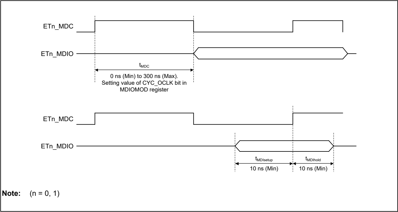
Figure 3.18 Management Interface
