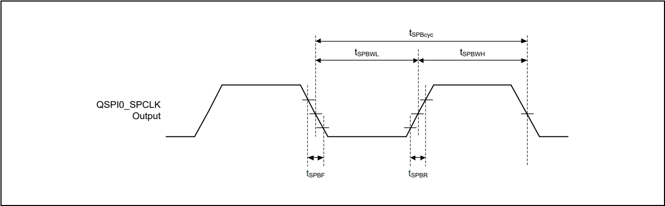
Figure 3.25 Clock Timing
