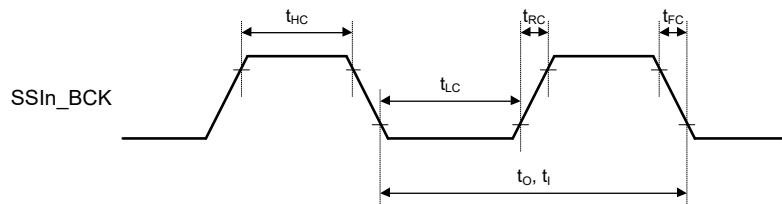
Figure 3.32 Bit Clock Input/Output Timing
