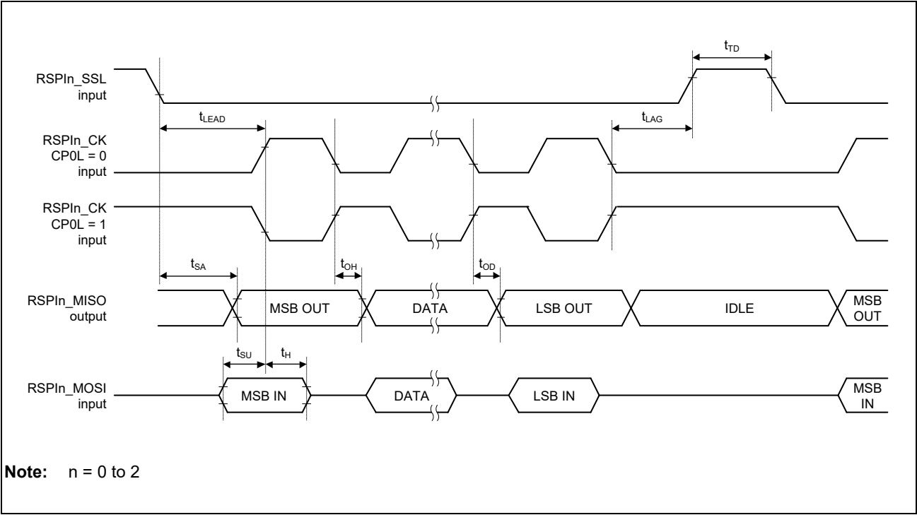
Figure 3.48 Transmission and Reception Timing (Slave, CPHA = 0)
