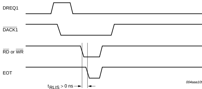
Fig 56. External EOT timing for HC single-cycle DMA.
