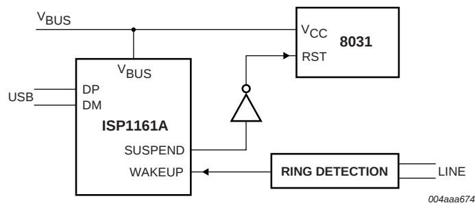
Fig 39. SUSPEND and WAKEUP signals in a powered-off modem application.
