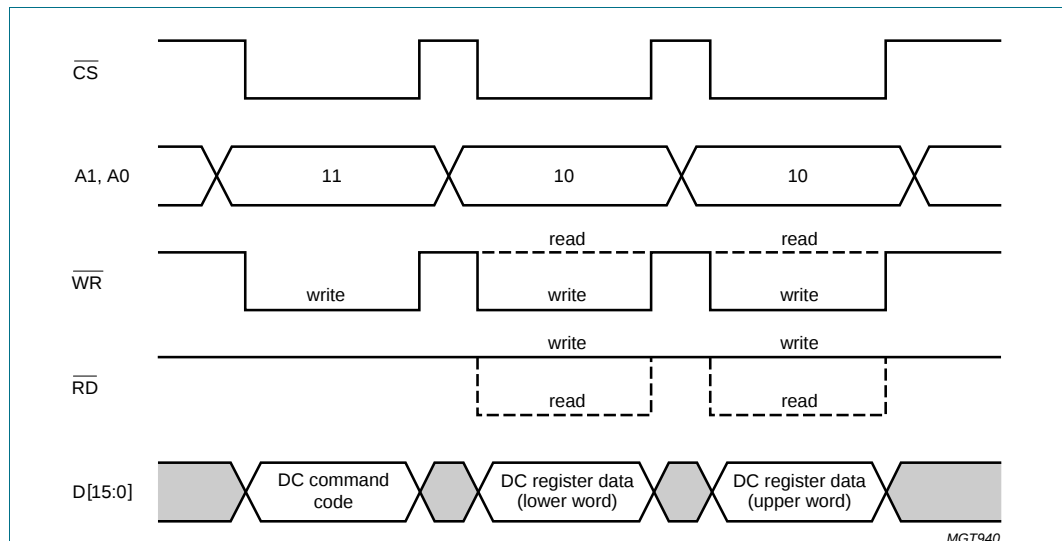
Fig 15. Accessing DC control registers.
