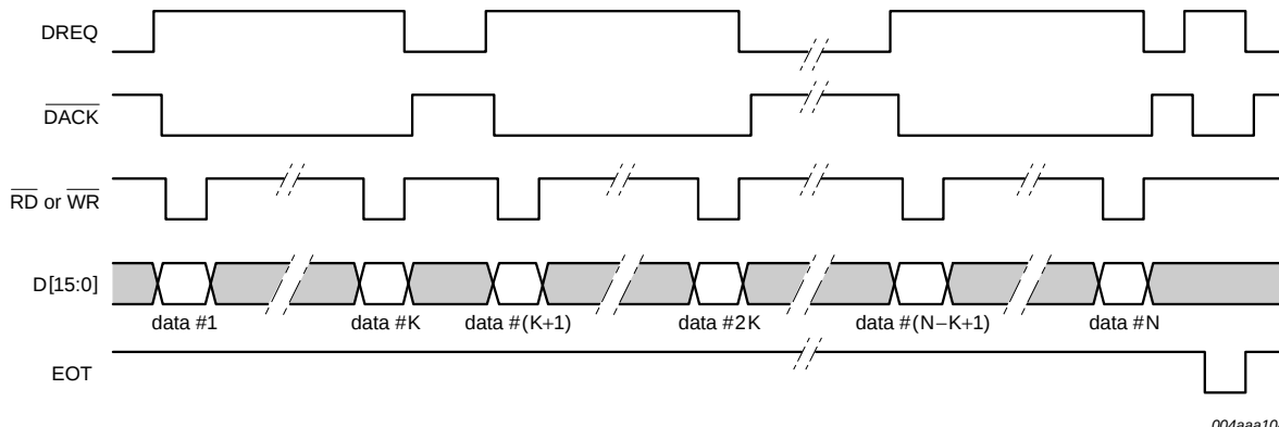
Fig 18. DMA transfer in burst mode.
