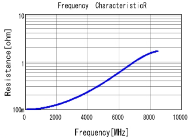
■ GCQ1555C1H6R0DB01 R DC0V, 25degC
