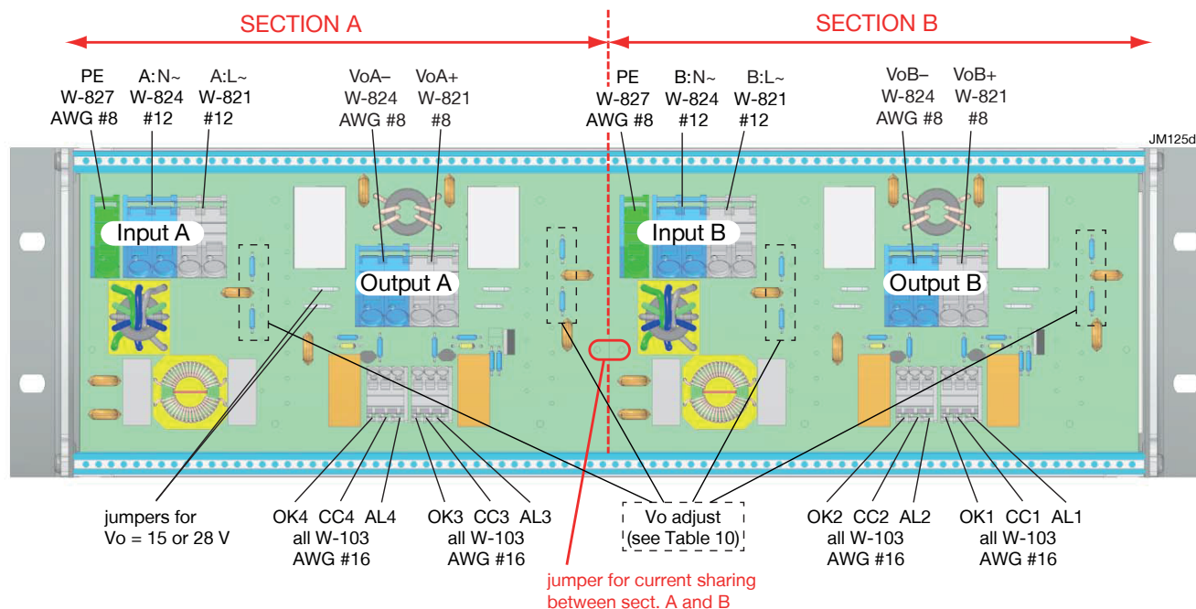
Fig. 13a: Rear view and connections of single output system.
