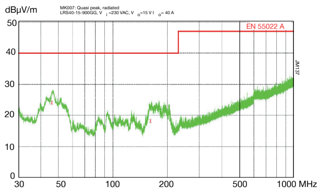
Fig. 10 Radiated emissions quasi peak, antenna distance 10 m (populated subrack system LRS40-15-900G at V_{in} = 230 VAC, V_o = 15 V, I_o = 40 A)
