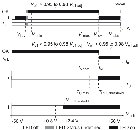
Fig.8 LED indicators
