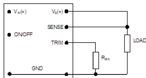
Circuit configuration to program output voltage using an external resistor
