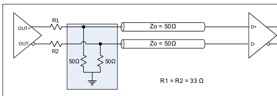
Figure 15. HCSL interface termination
