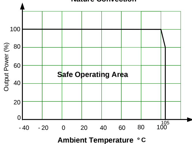
Other models Nature Convection
