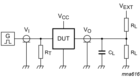
b. Test circuit
