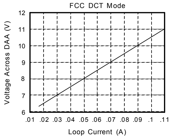
Figure 20. FCC Mode I/V Characteristics
