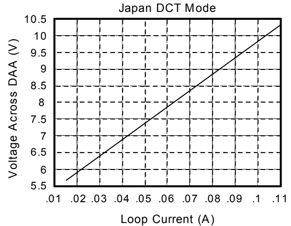
Figure 22. Japan Mode I/V Characteristics
