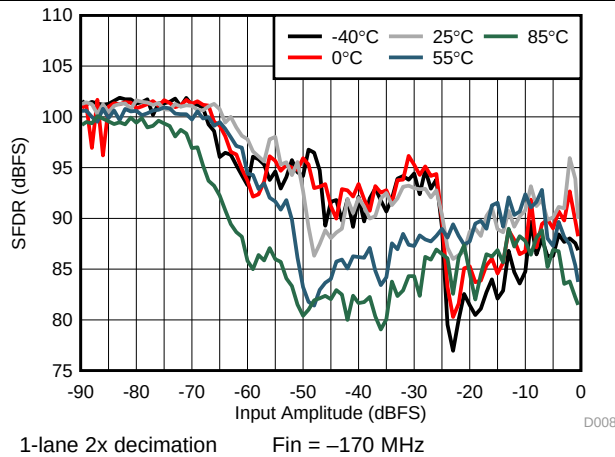
Figure 12. SFDR vs. Amplitude
