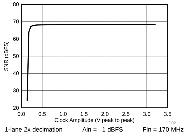
Figure 25. SNR vs. Clock Amplitude
