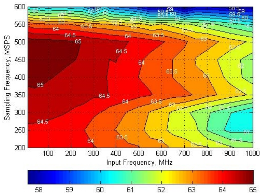
Figure 37. SNR Contour Plot
