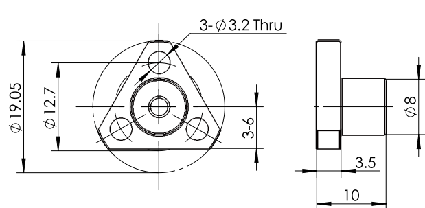
Triangular Standard Nut AT0
