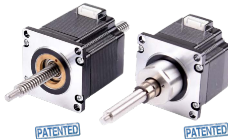
Non-Captive Shaft
