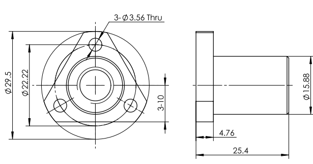
Triangular Standard Nut AT2
