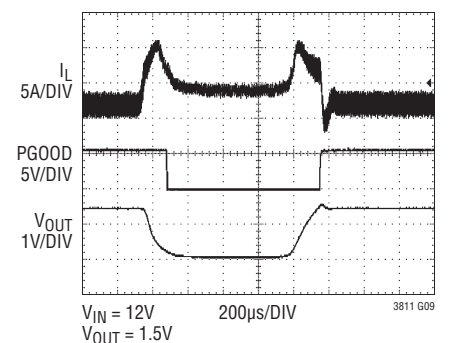
Short-Circuit Waveforms
