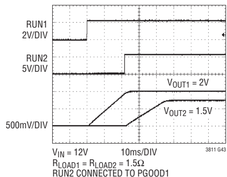
Sequenced Start-Up
