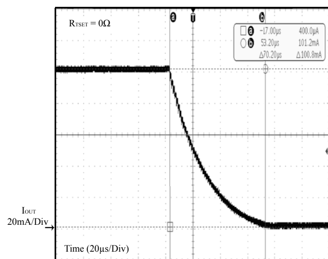
Figure 13 Instant Off
