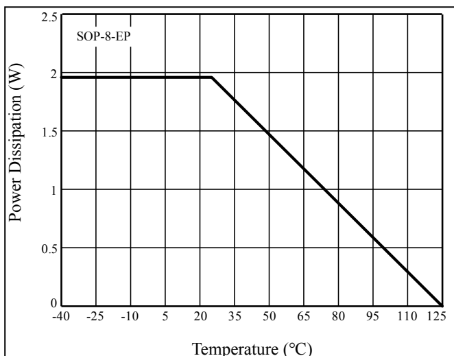
Figure 28 Dissipation Curve
