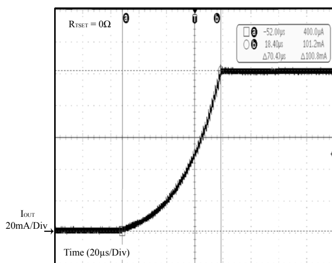
Figure 12 Instant on
