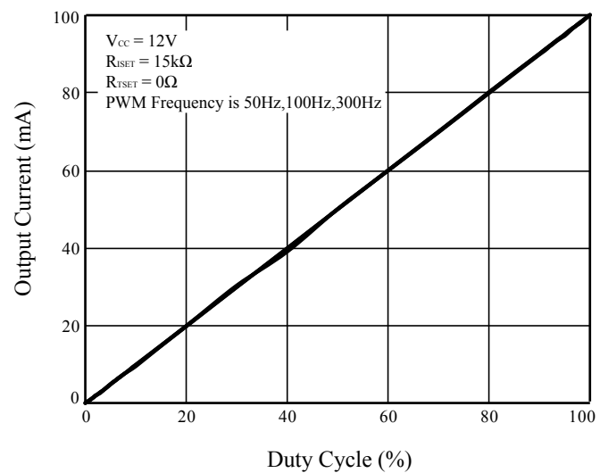
Figure 5 Output Current vs. PWM Duty Cycle
